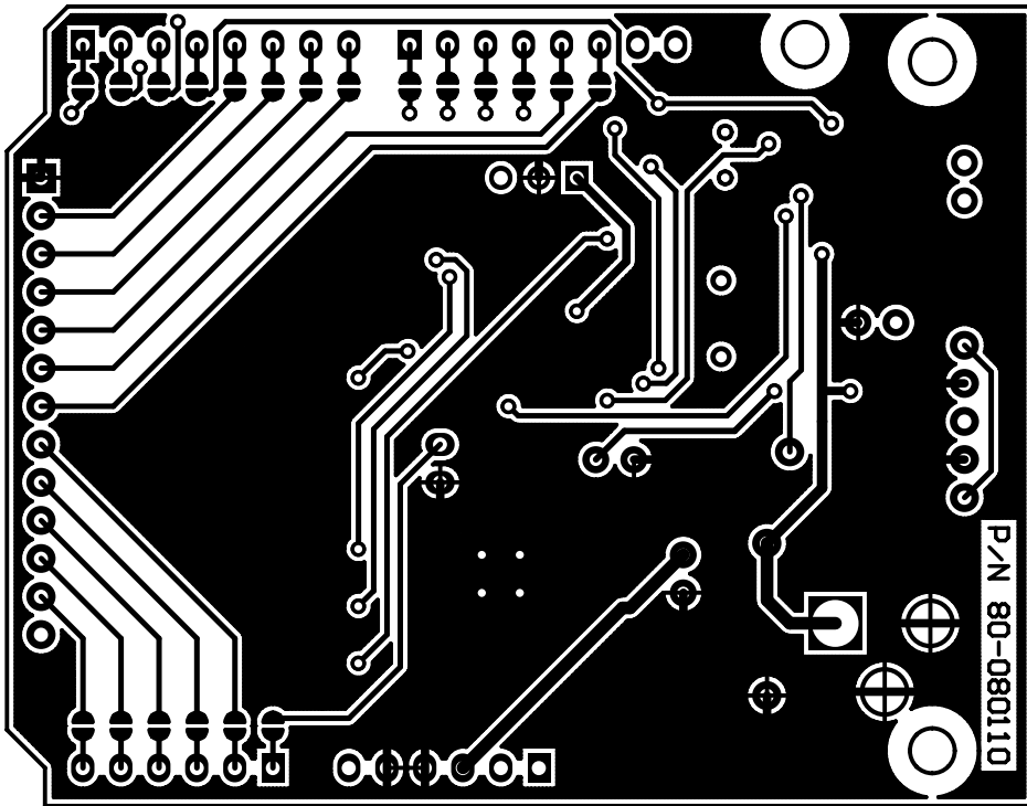
11 Function IR wireless remote control kit Copper Pattern Layout (Bottom Layer)
