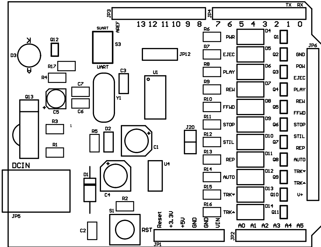
11 Function IR wireless remote control kit Silk Screen Layout
