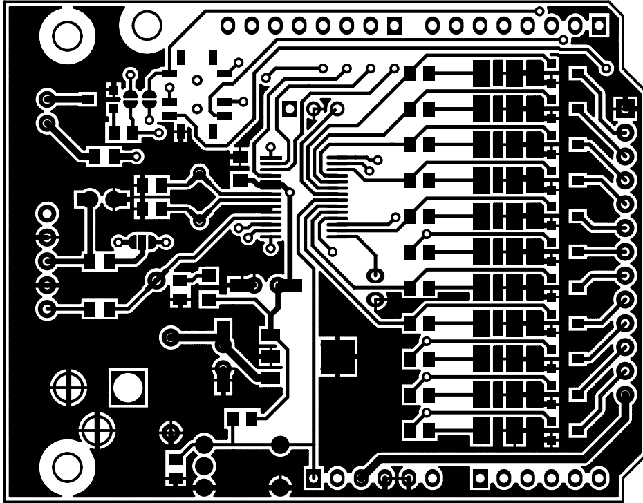
11 Function IR wireless remote control kit Copper Pattern Layout (Top Layer)
