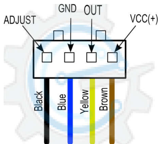
Figure 1. Liquid level detector pinouts
