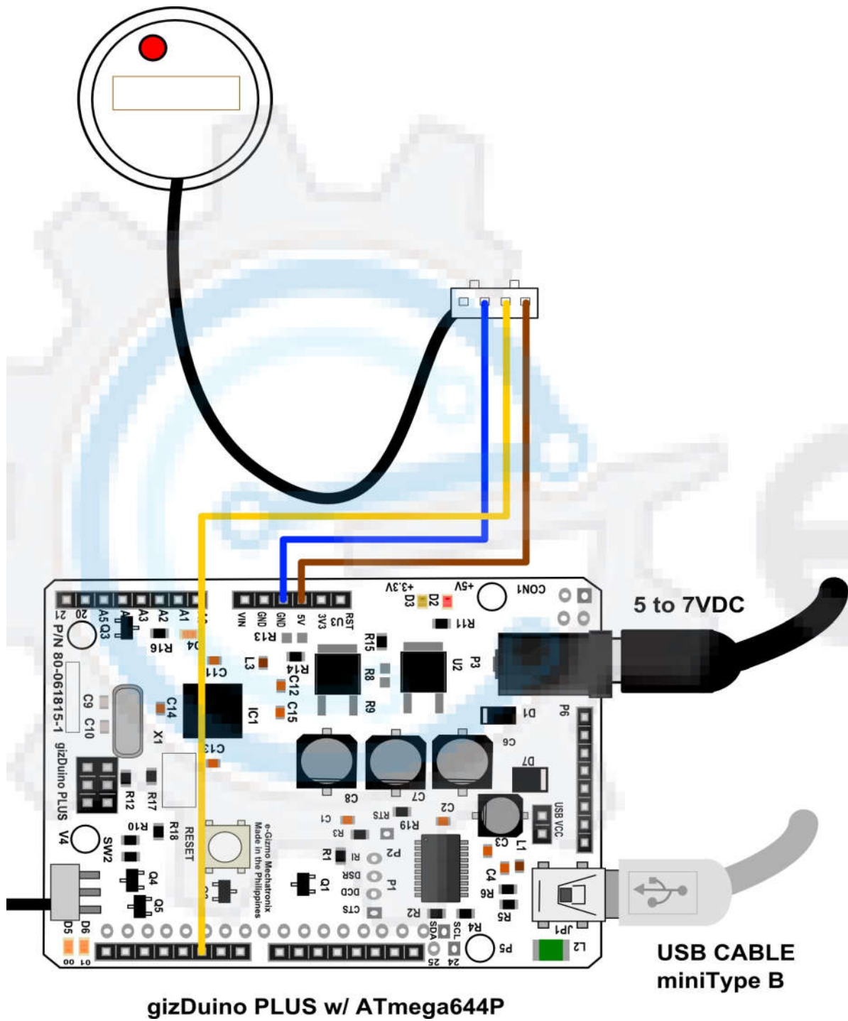
Figure 2. Sample connections
