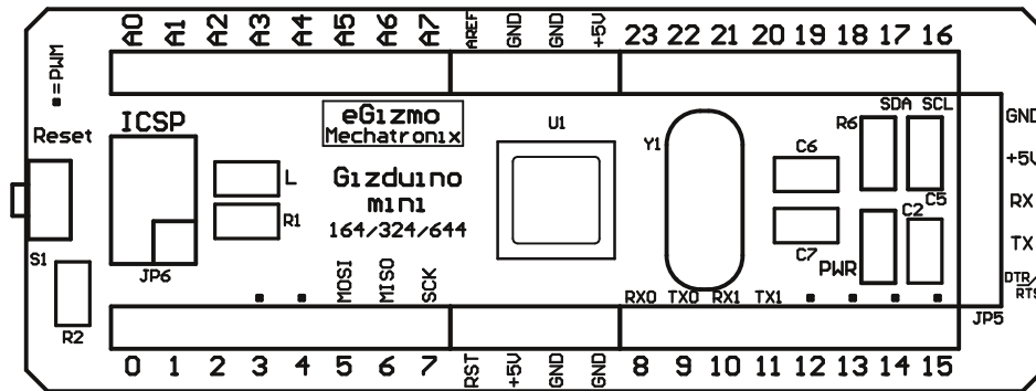
Figure 3. Parts Placement
